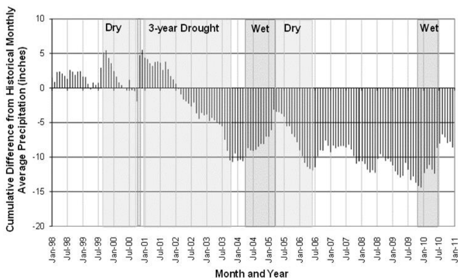
Figure 1 Cumulative difference from historic monthly mean
