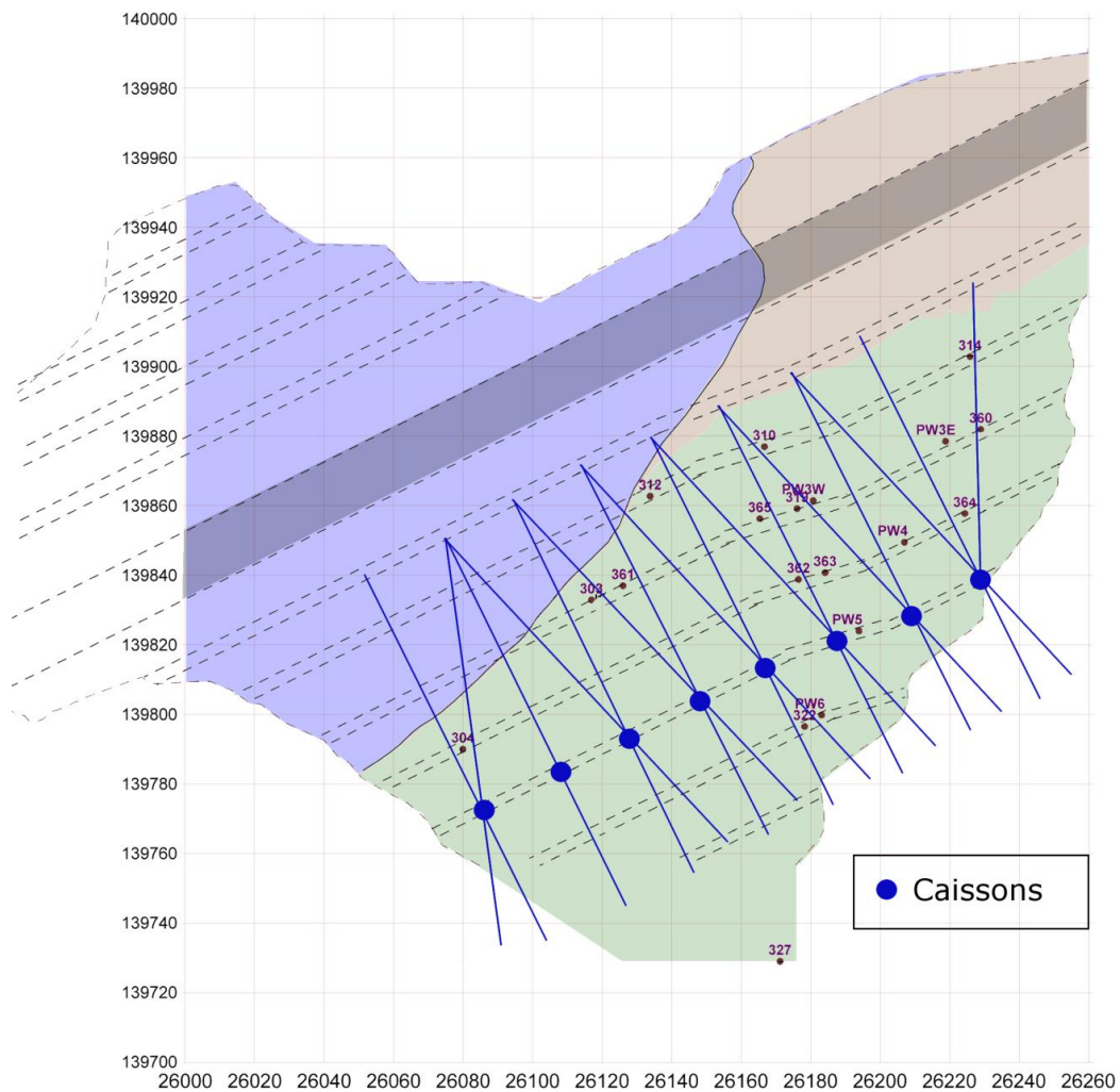
Figure 6 The favoured design using drilled dipping drains that pass through pumped caissons
