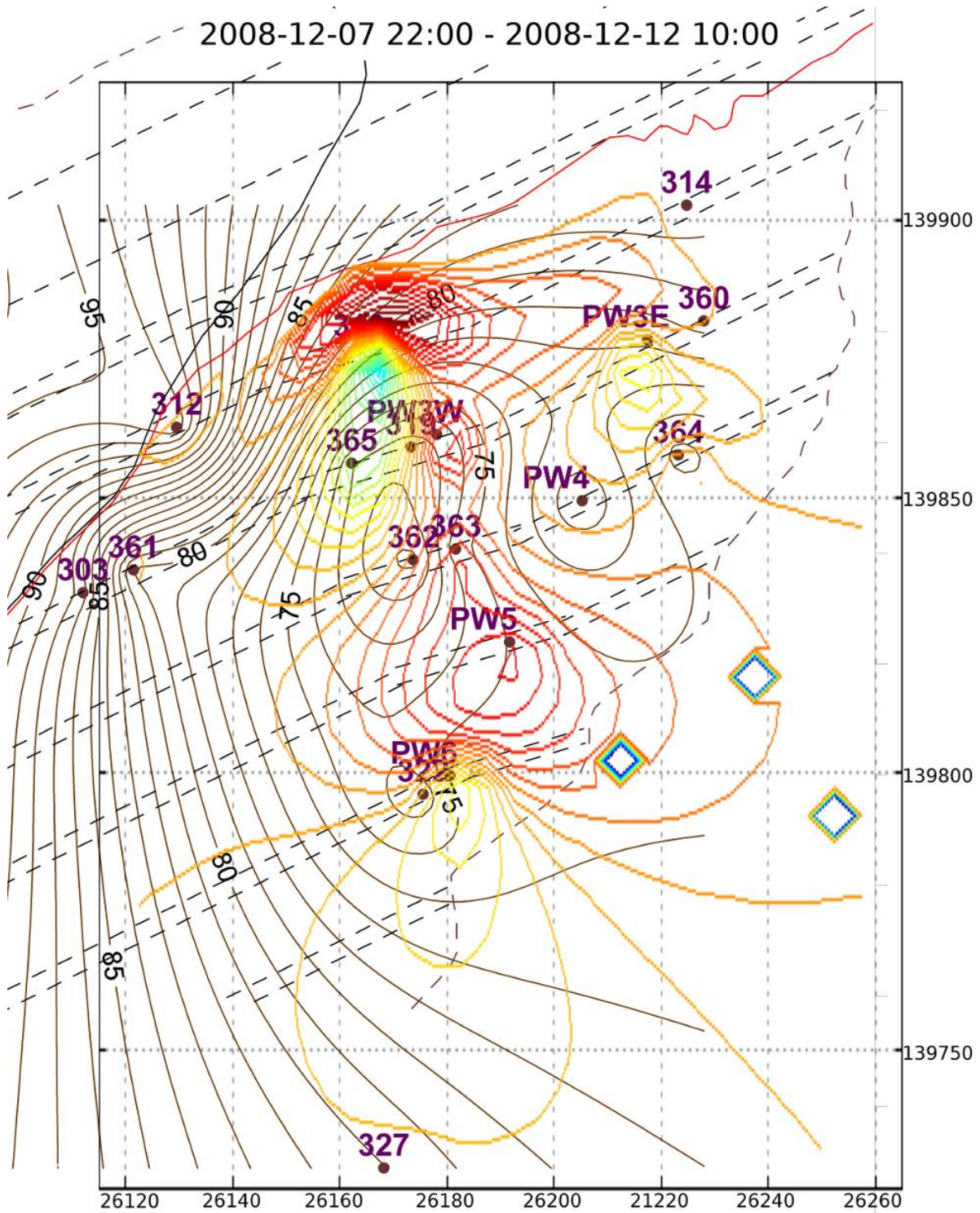
Figure 5 The net calculated imbalance (mm) in the period from 2200 hrs on 7 December 2008 to 1000 hrs on 12 December 2008 corresponding to time steps 8 to 9 on Figure 3. During this period 41 mm of rain fell and pumping tests were conducted on the four wells 3E, 3W, 4 and 5
