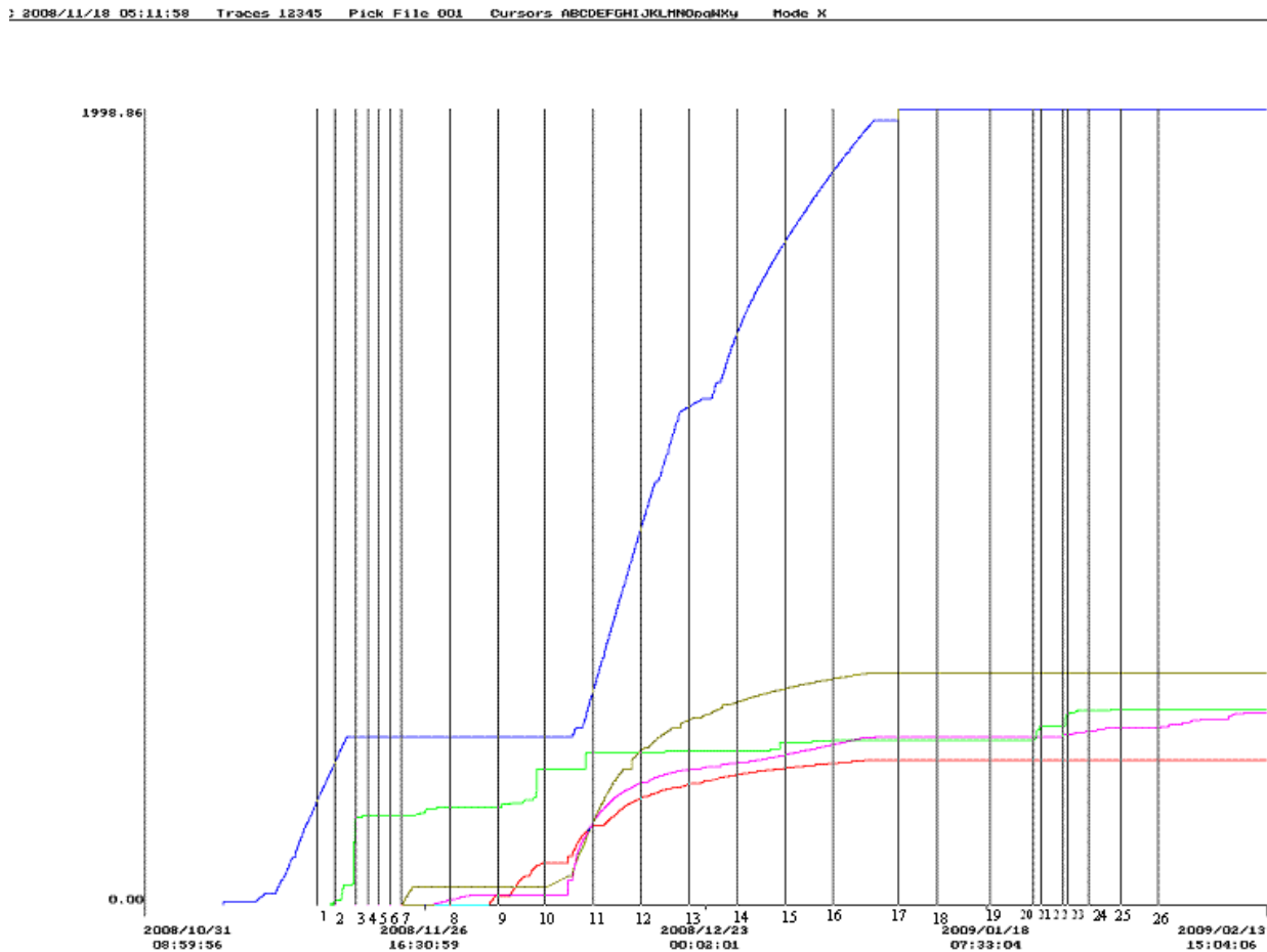
Figure 3 Cumulative plot of pumping on cut 3 with rainfall information. The numbers on the abscissa refer to specific time steps. Blue = pump well 5, green = rainfall, brown = pump well 4, purple = pump well 3E, Red = pump well 3W
