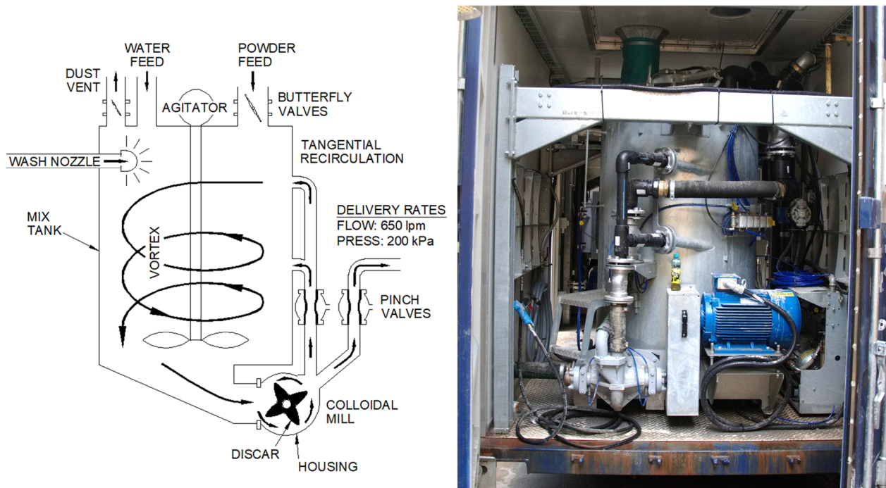
Figure 7 Binder slurry plant colloidal mixer
