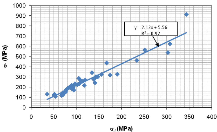
Figure 8 Sigma 1 versus sigma 3 values obtained from analysis
