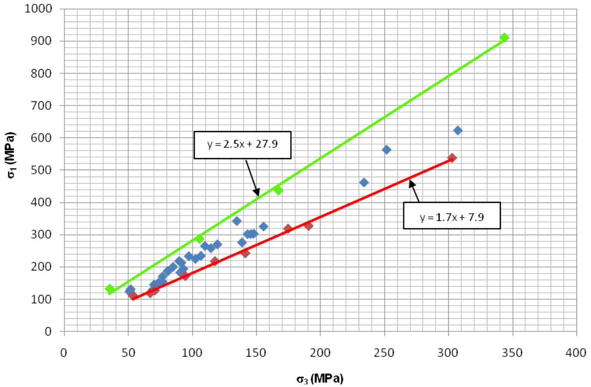
Figure 9 Upper and lower limit trend lines obtained from the analyses
