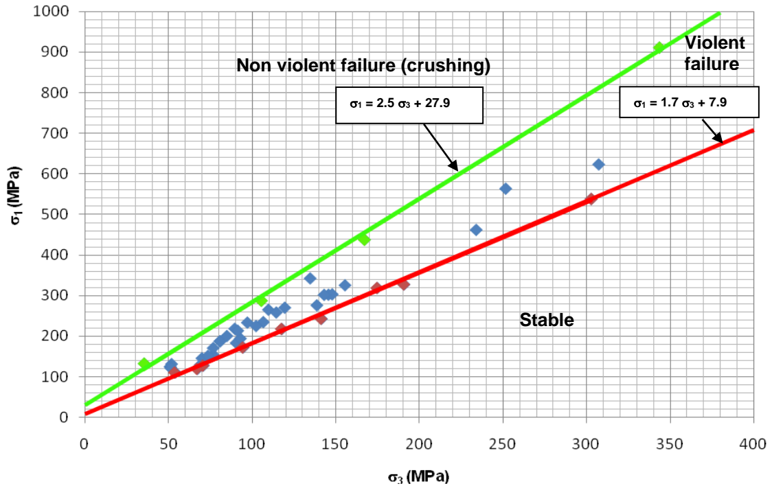
Figure 10 Upper and lower limits for remnant failure in the Free State
