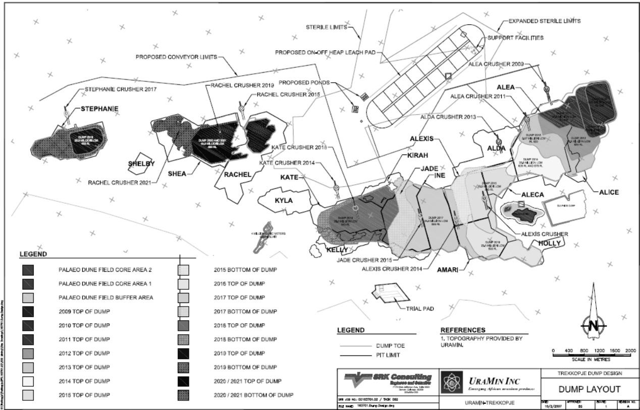
Figure 3 Mining surface infrastructure and final dump locations (SRK, 2008)
